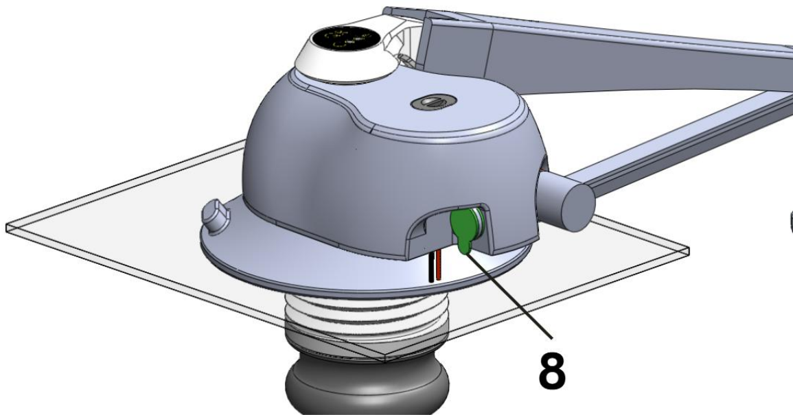
Figure 1: GeckoWiper key components, 1.) Geckowiper housing, 2.) Vacuum pump plunger indicator, 3.) Wiper arm, 4.) Wiper blade, 5.) Vacuum pad, 6.) Remote transmitter, 7.) Safety magnet, 8.) USB-C charging port with silicone waterproofing cover
